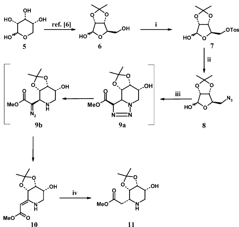
Scheme 1. (i) TosCl, pyridine; (ii) \text{NaN}_3 , DMSO; (iii) \text{Ph}_3\text{P}=\text{CHCO}_2\text{CH}_3 , \text{Rh}_2(\text{OAc})_4 , \text{Et}_3\text{N} , \text{CH}_2\text{Cl}_2 ; (iv) \text{H}_2 , Pd/C, \text{CH}_3\text{OH} .
